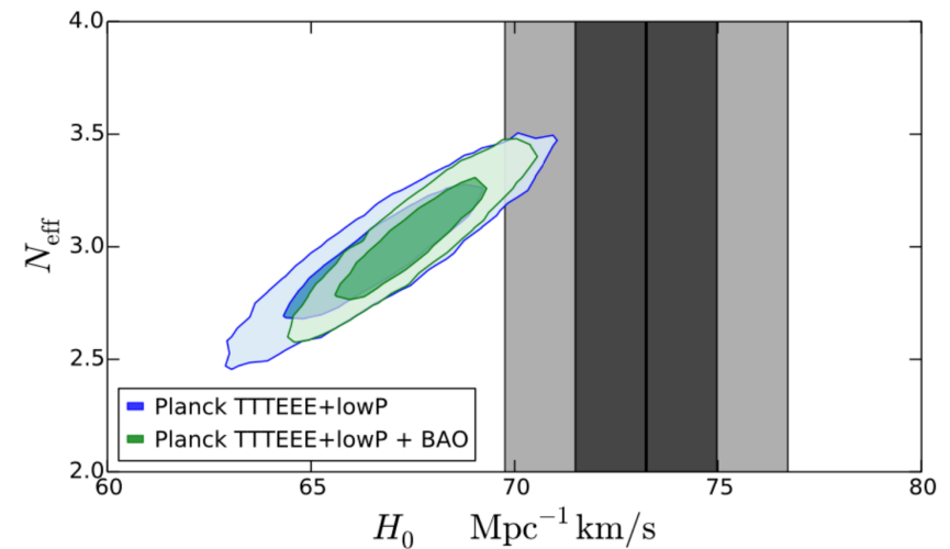
Figure: reference arXiv:1607.05617 [astro-ph.CO]
